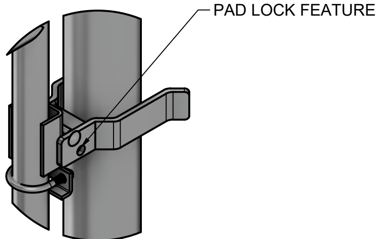
LATCH DETAIL B
